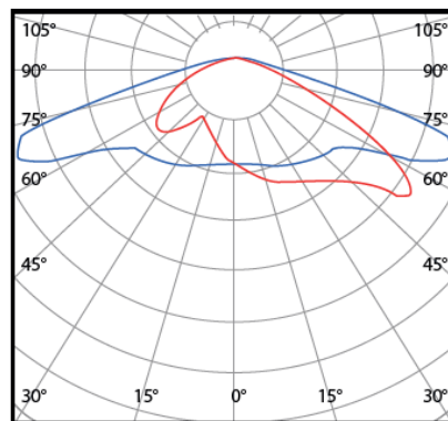
cd/klm — C0 - C180 — C90 - C270
